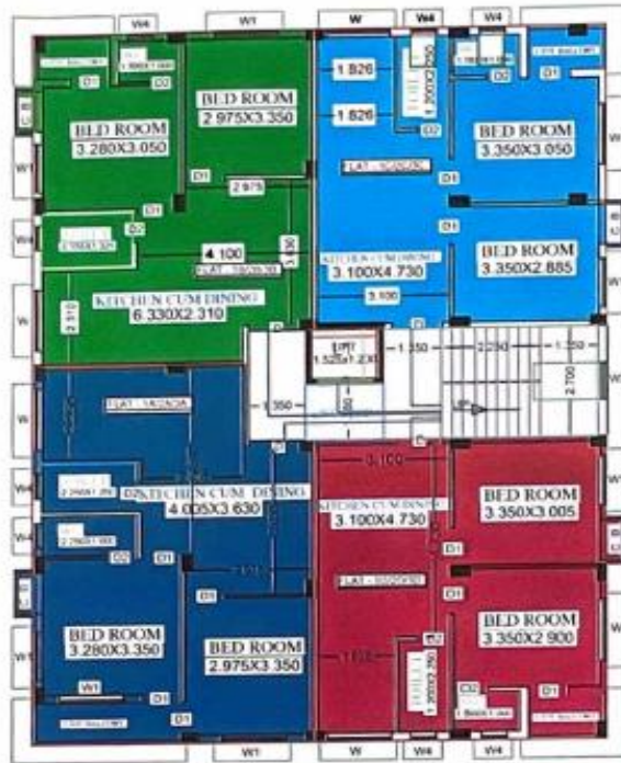
Typ. (1st, 2nd, 3rd) FLOOR PLAN FLOOR01,FLOOR02,FLOOR03,-TYPICAL
